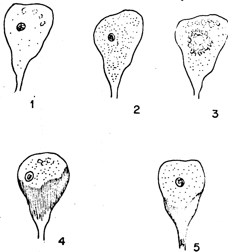
.FIG. 21 Different stages of neurosecretory activity in the NSC of Perna indica and Perna viridis as deduced from their staining property. The stages 1-5 are arbitrary as the process of NSM secretion, accumulation and evacuation is continuous in a given cycle of activity.
