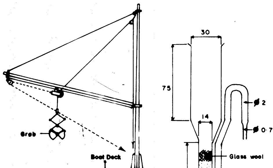
* FIG. F-1: System for hoisting grab using jockey pulley
