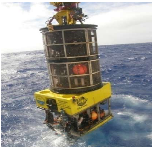
ROV ROSUB 6000 deployment
