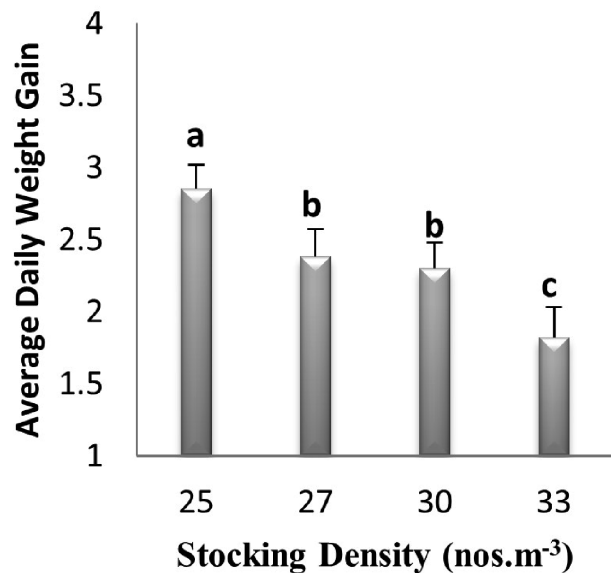
Fig. 6. Average daily weight gain (ADWG) of Asian seabass cultured under different stocking densities. Mean values and standard error (mean \pm SE) is presented. Different superscripts in the bar diagram indicate significant differences among different stocking densities (One way ANOVA, Tukey's Post-Hoc, p < 0.05 )
