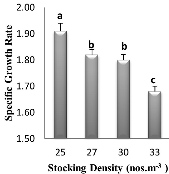
Fig. 5. Specific growth rate (SGR) of Asian seabass cultured under different stocking densities. Mean values and standard error (mean \pm SEM) is presented. (One way ANOVA, Tukey's Post-Hoc, p < 0.05 )
