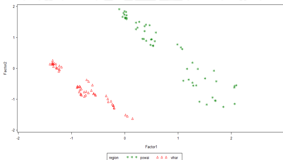
Figure 3: Score plot between the first and second factors based on the physico-chemical parameters for Powai and Vihar. A total of 34 genera of phytoplankters were observed in Powai Lake whereas it was 51 in Vihar (Table 5).
