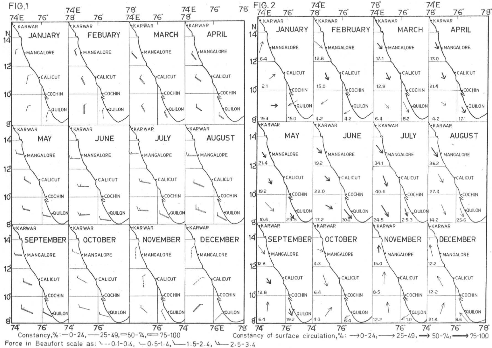
Fig. 2 — Monthly resultant surface currents in 2° square along SW coast of India [Values give current velocity in cm/sec]
