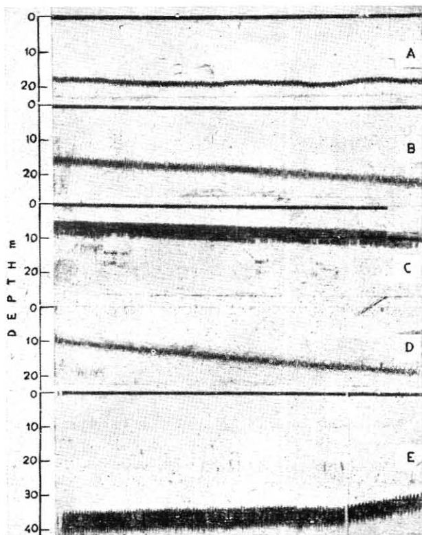
Fig. 7 — Echograms of the Alleppey mud bank and of mud bottom. Distance covered in all the recordings is 4 km. For all recordings, the gain of the recorder was kept constant [A, echo traces of the bottom of a non-mud bank area during the non-monsoon months. B, echo traces of the same area during the monsoon months. C, echo traces of a mud bank when it became fully active. Difference in the structure of the deposit is seen when the 'white line' was switched on towards the end of the record. D, echo traces of a non-mud bank area during the monsoon months with the 'white line' on. E, echogram taken off Nircunnam where thick mud was found at depths of 30-40 m]
