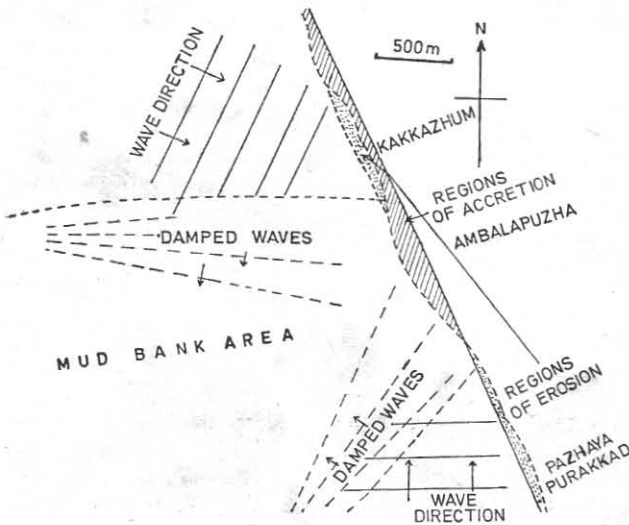
Fig. 12 — Shoreline changes induced by the presence of mud bank near Ambalapuzha during 1972 [Both southern and northern areas adjacent to mud bank get eroded, but the erosion is severe on the southern side, probably because of the proximity of a seawall nearby. Wave directions have been shown by large arrows. Damped waves within the mud bank are indicated by smaller arrows]
