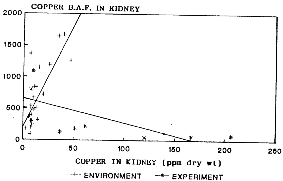
FIG. 15. Relationship between Bioaccumulation and Bioaccumulation Factor (B.A.F.) of copper in Kidney of L. persia .
