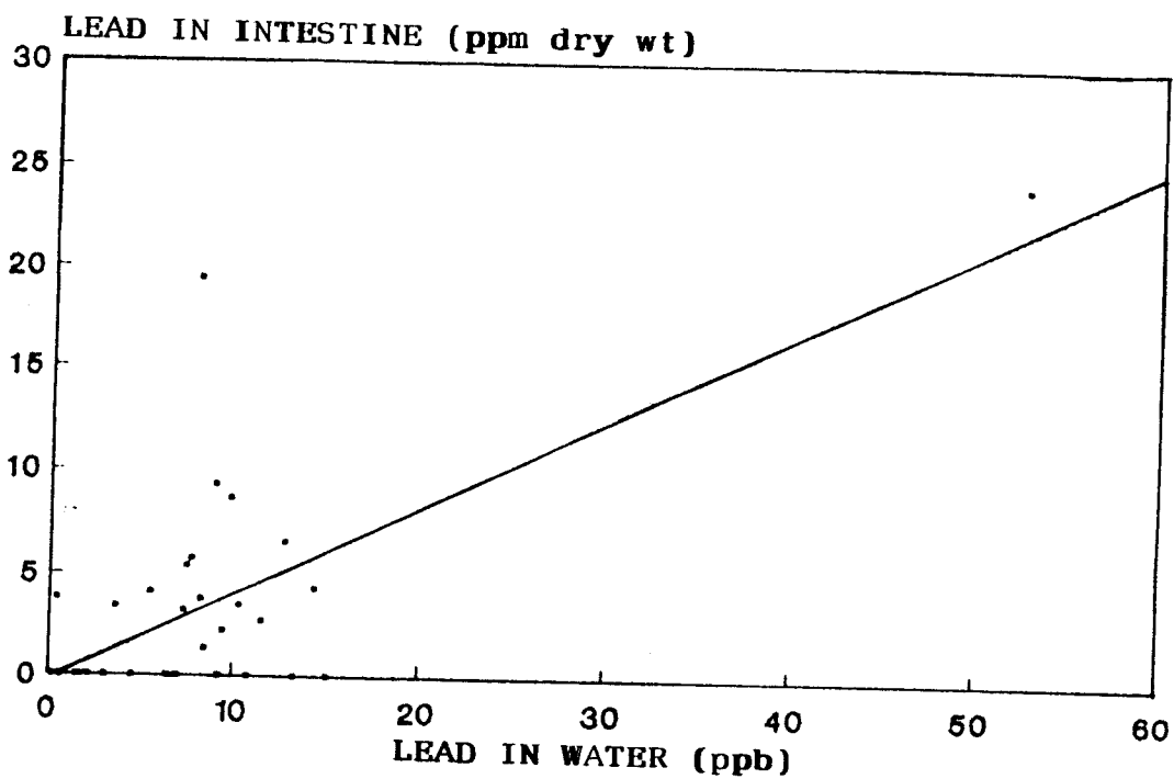
FIG. 5. Relationship between lead in Water and lead in intestine of L. parsia
