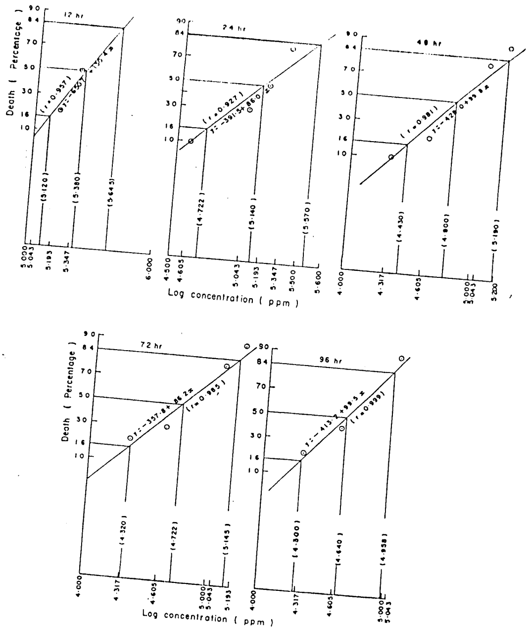
FIG. 12. Response curve of lead nitrate at 12, 24, 48, 72 and 96 hours
