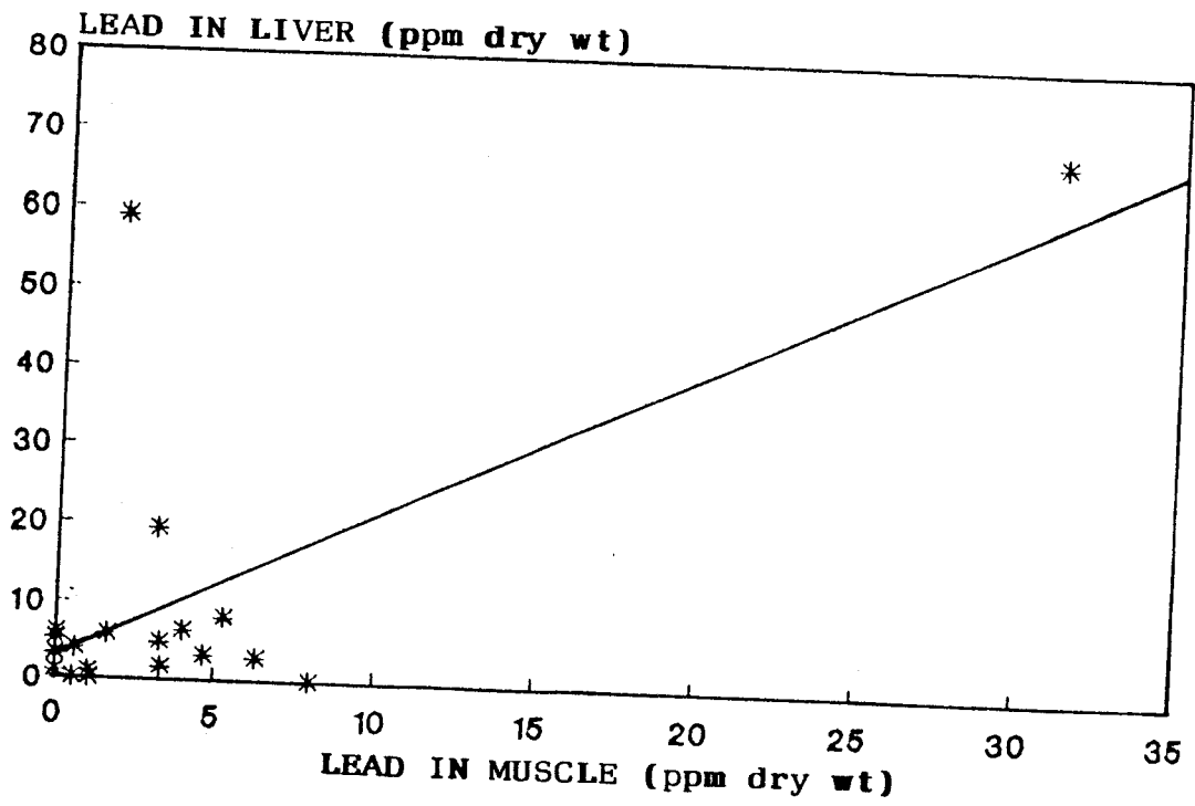
FIG. 7. Relationship between lead in Muscle and lead in Liver of L. parsia .
