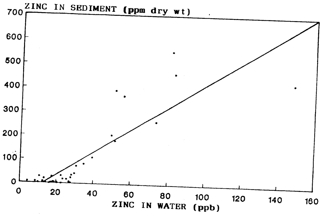
FIG. 4. Relationship between zinc in Water and zinc in Sediment.
