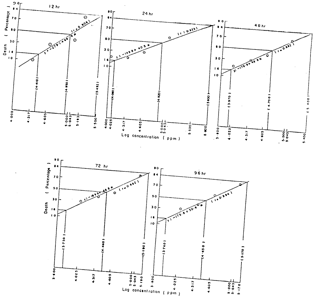
FIG. 10. Response curve of copper sulphate at 12, 24, 48, 72 and 96 hours
