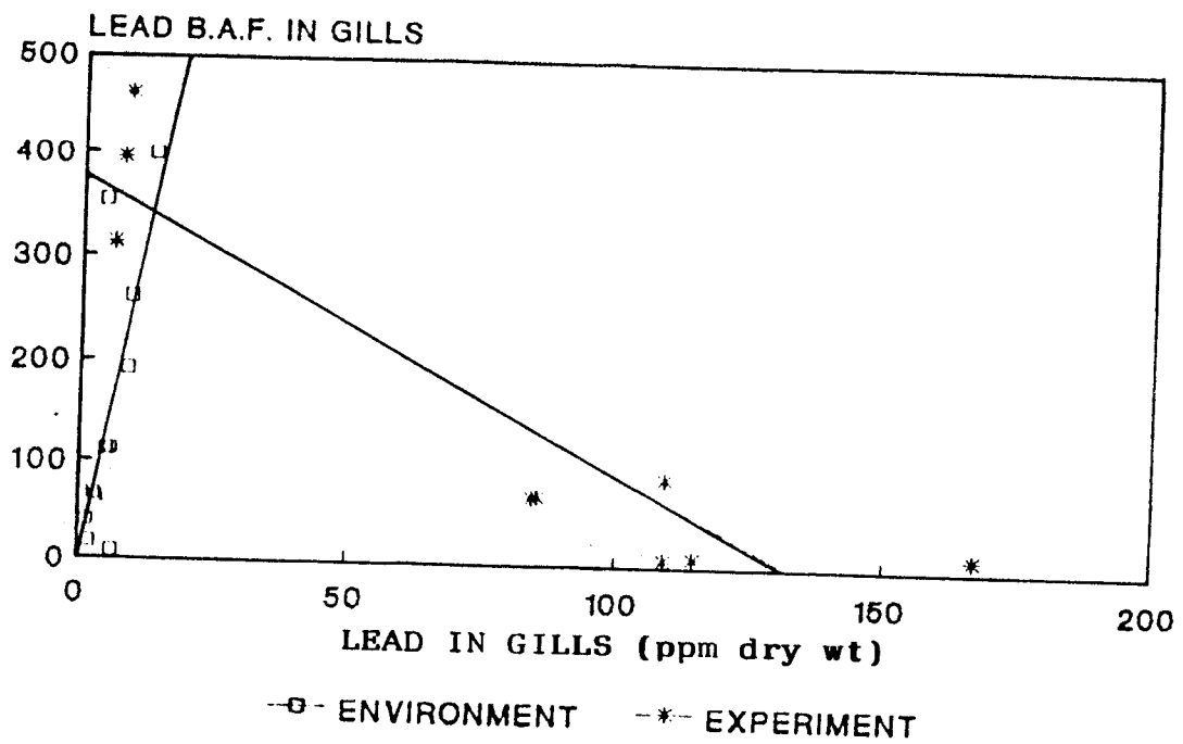
FIG. 17. Relationship between Bioaccumulation and Bioaccumulation Factor (B.A.F.) of lead in Gills of L. parsia .
