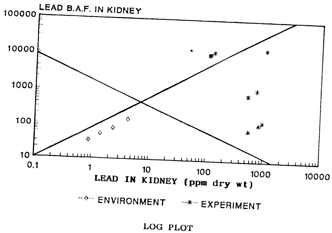
FIG. 18. Relationship between Bioaccumulation and Bioaccumulation Factor (B.A.F.) of lead in Kidney of L. persia .
