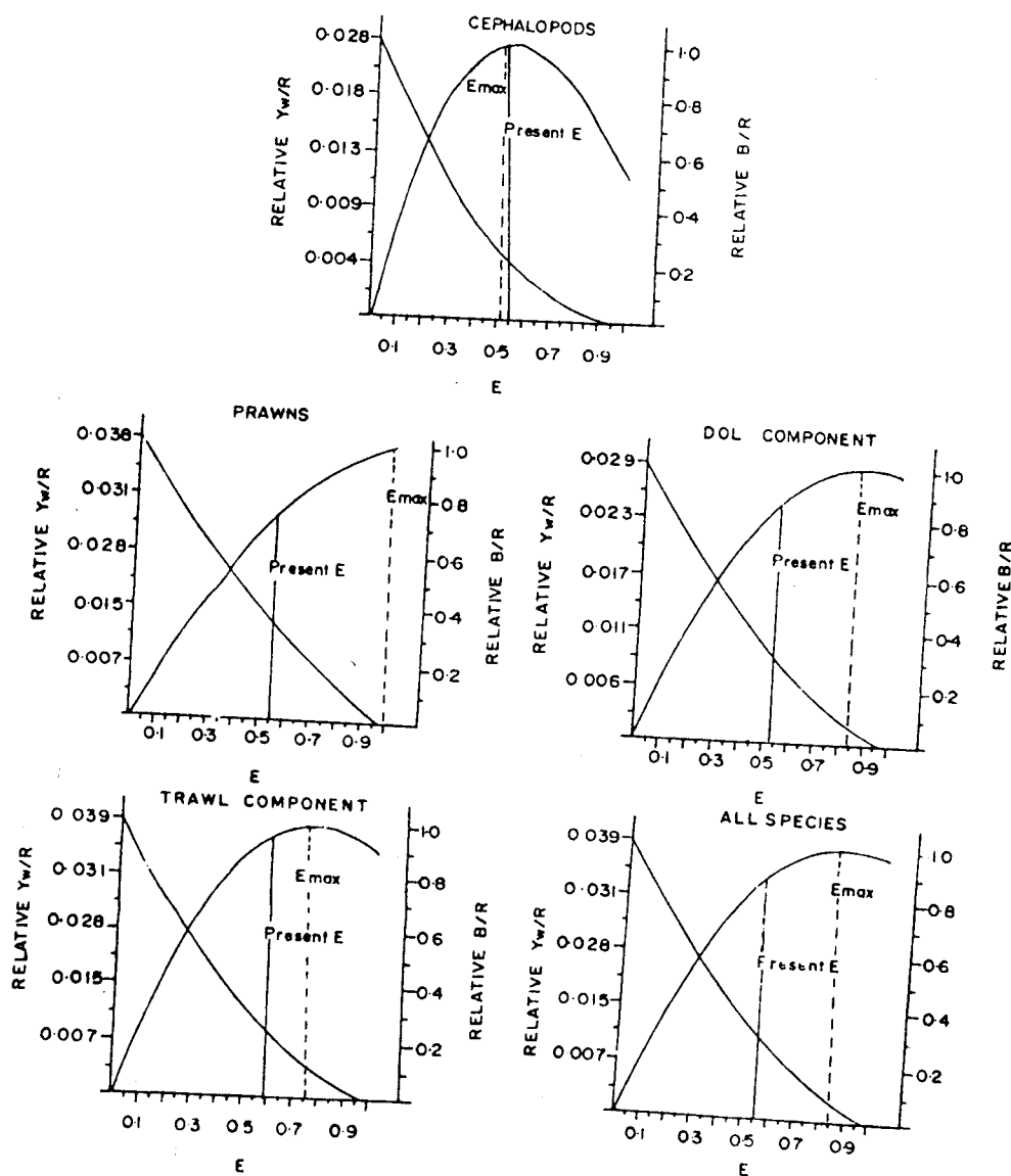
Fig. 1—Gear wise estimates of relative yield per recruit and biomass per recruit for various resources
