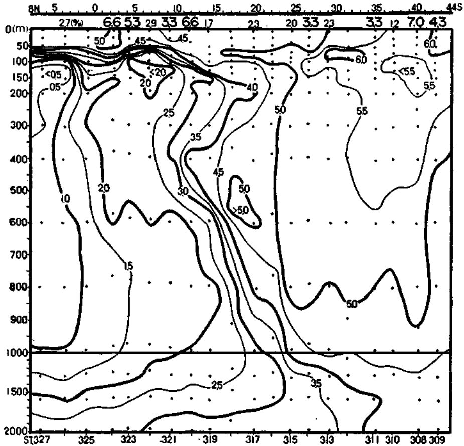
Fig. 7c. Vertical distribution of dissolved oxygen (ml/l), along 75° E.-line, Apr. 4-30, 1964 Figures along 0 m-line indicate hook rate (%) by the long-line at each station.
