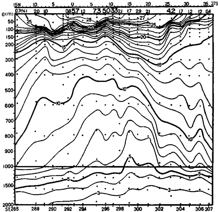
Fig. 6a. Vertical distribution of water temperature (°C), along 55° E. - line, Feb. 5- Mar. 9, 1964. Figures along 0 m-line indicate back rate (%) by the long-line at each station (See Fig. 1)
