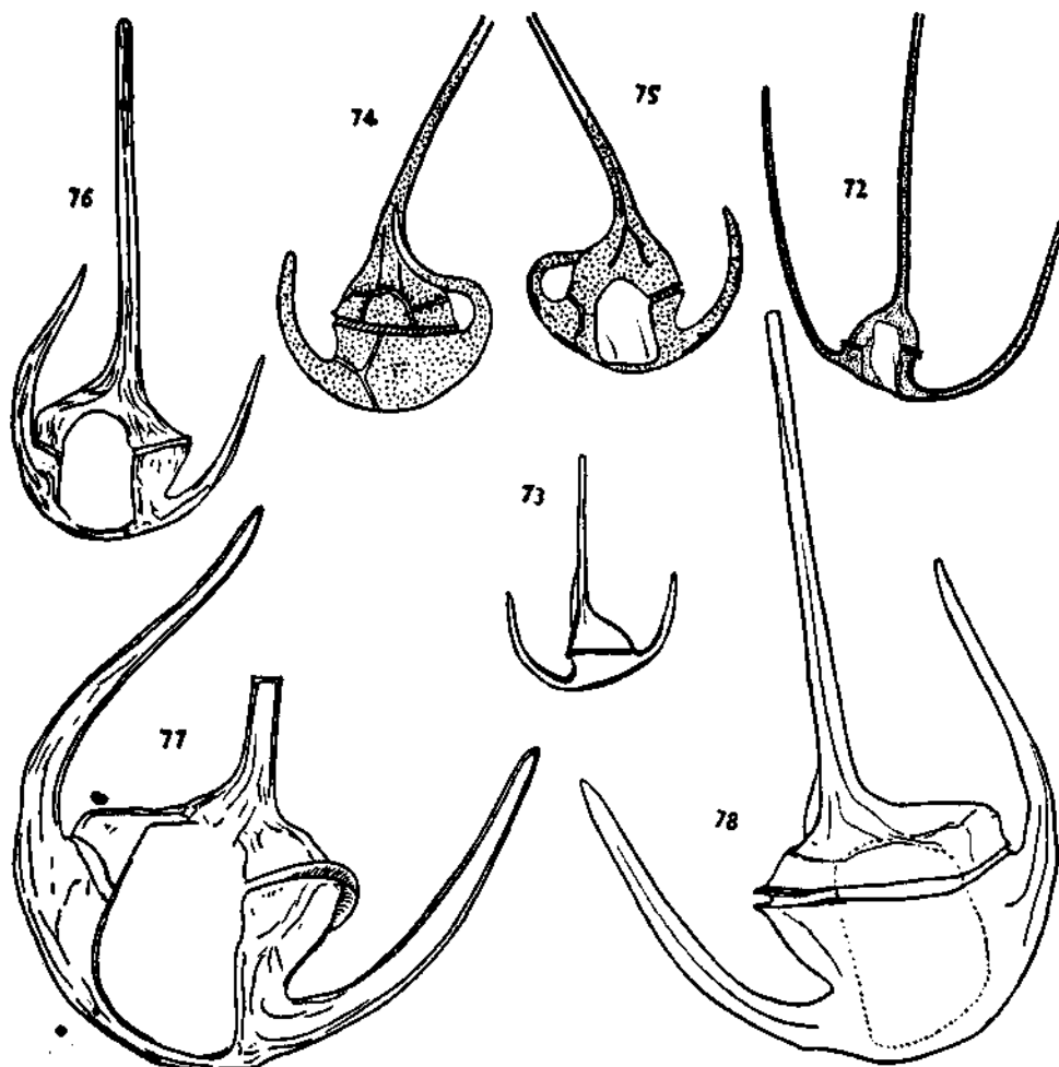
Text-figures. 72-78. Fig. 72, 73— Ceratium karstenii f. robustum (Karsten) Jörgensen; ventral and dorsal views; (72, after Schiller 73, from Schiller 1937). Figs. 74, 75— C. conciliens Jörgensen; dorsal and ventral views; (after Schiller, 1937). Figs. 76, 77, 78— C. gibberum Gourret. 76, 77, ventral views, 78, dorsal view; (original). (72, x 100; 73, x 95; 74, 75, x 210; 76, x 180; 77, 78, x 380).
