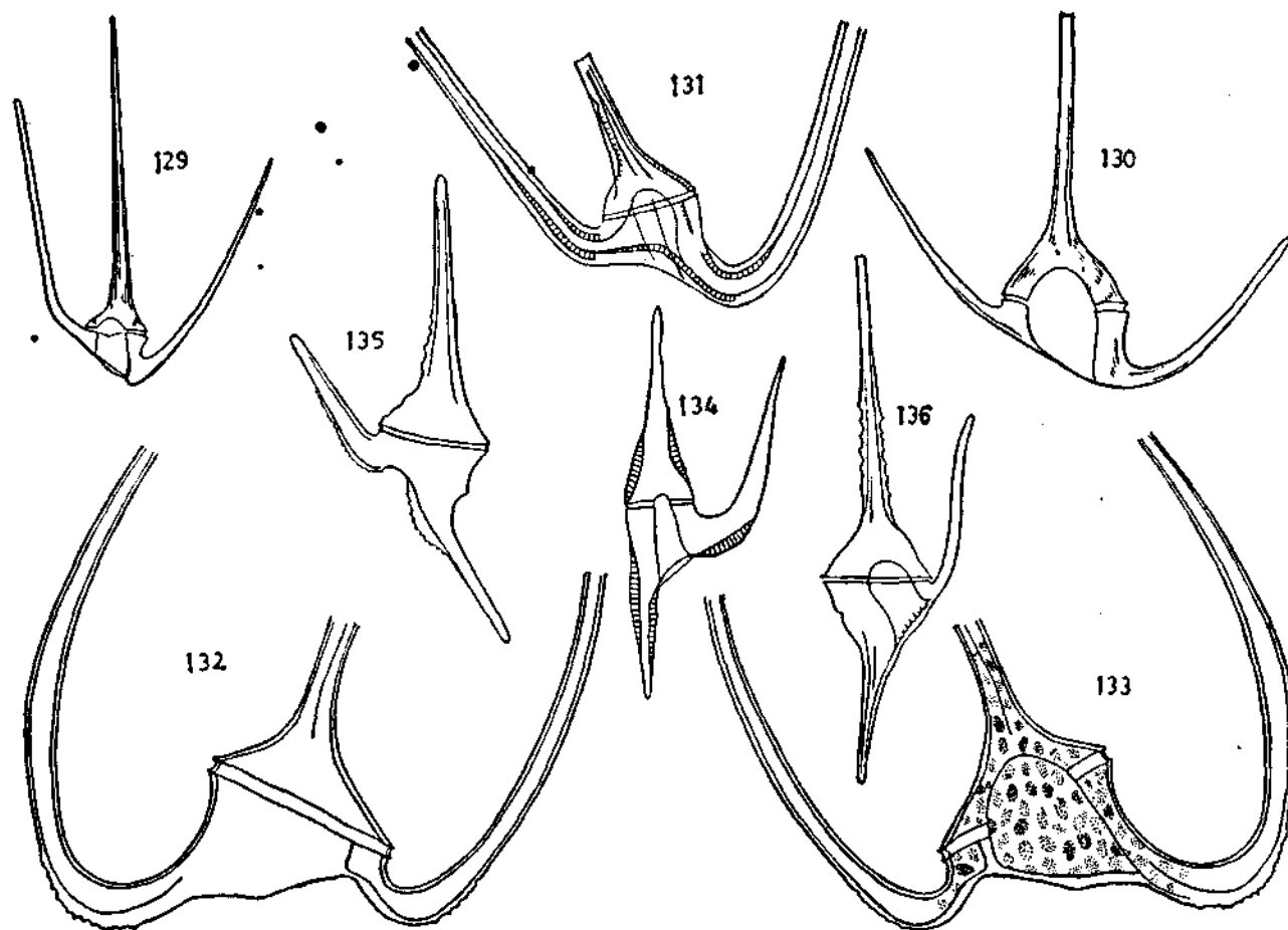
Text-figures 129-136. Figs. 129, 130 - Ceratium pavillardii Jörgensen. ventral views; (129, after Jörgensen, 1920; 130 from Schiller). Fig. 131 - C. vultur Cleve; ventral view; (after Cleve, 1900). Figs. 132, 133 - C. vultur var. sumatranum (Karsten) Steemann Nielsen; dorsal and ventral views; (original). Fig. 134 - C. vultur var. productum Wood; ventral view; (after Wood, 1963b). Figs. 135, 136 - C. reflexum Cleve; dorsal and ventral views; (after Cleve, 1900). (129, x 200; 131, 132, 133, 135, 136, x 250; 130 and 134, not given).
