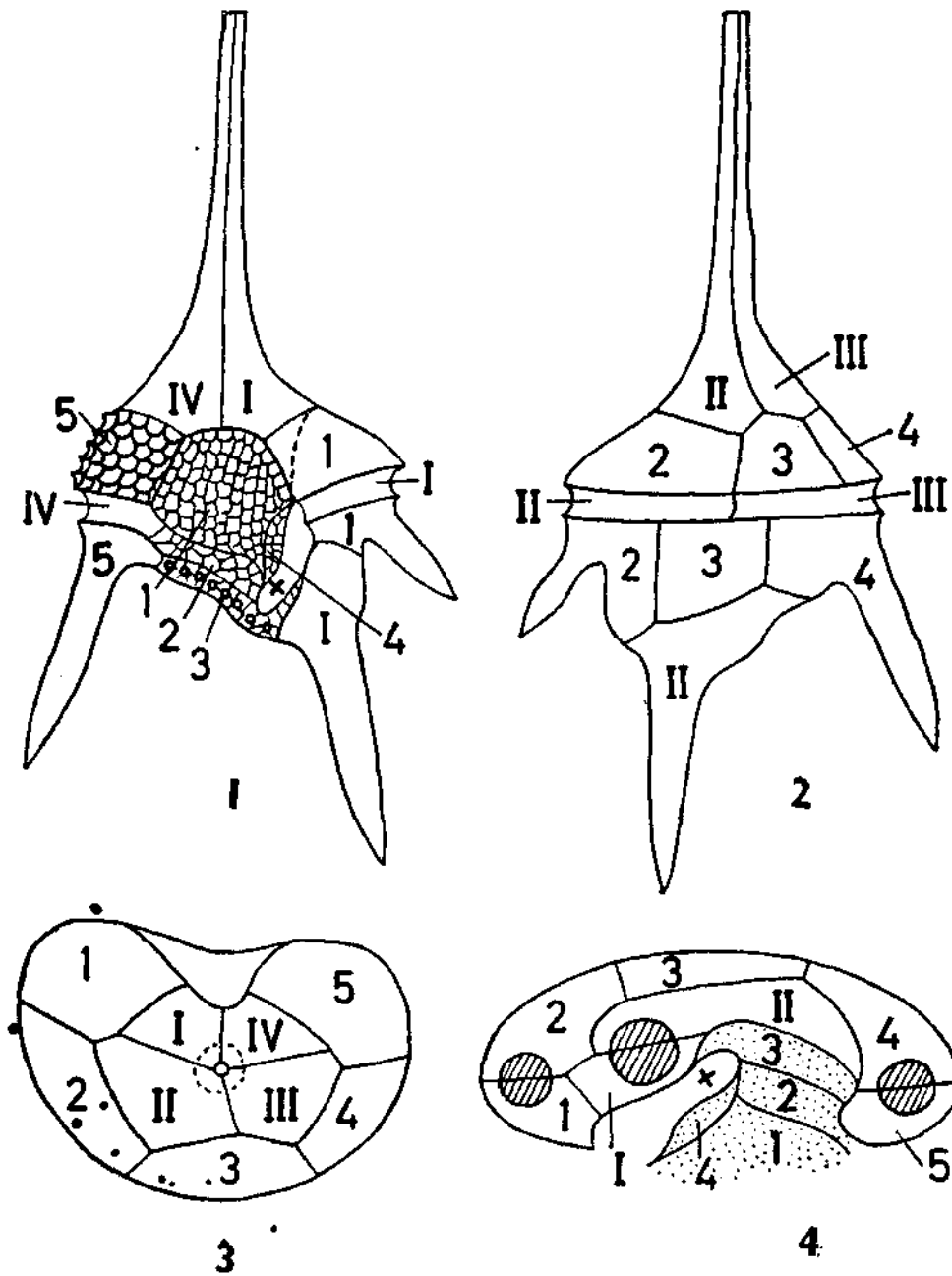
Text Figures 1-4. Ceratium hirundinella (O F Müller) Bergh. 1. Ventral view; the plates of the longitudinal furrow region (section through body) are strongly bordered by the longitudinal furrow (x). 2. Dorsal view 3. Epitheca plan (the anterior horn indicated by dots). 4. Hypotheca plan, (the three posterior horns are indicated by hatching the plates of the longitudinal furrow region set out by dots, the longitudinal furrow pointed out by a 'x' sign). In all the figures the apical -, transverse furrow - and antapical - plates are designated by roman, - the pre - and post - equatorial plates with arabic numerals correspondingly. (After Lindemann, 1928).
