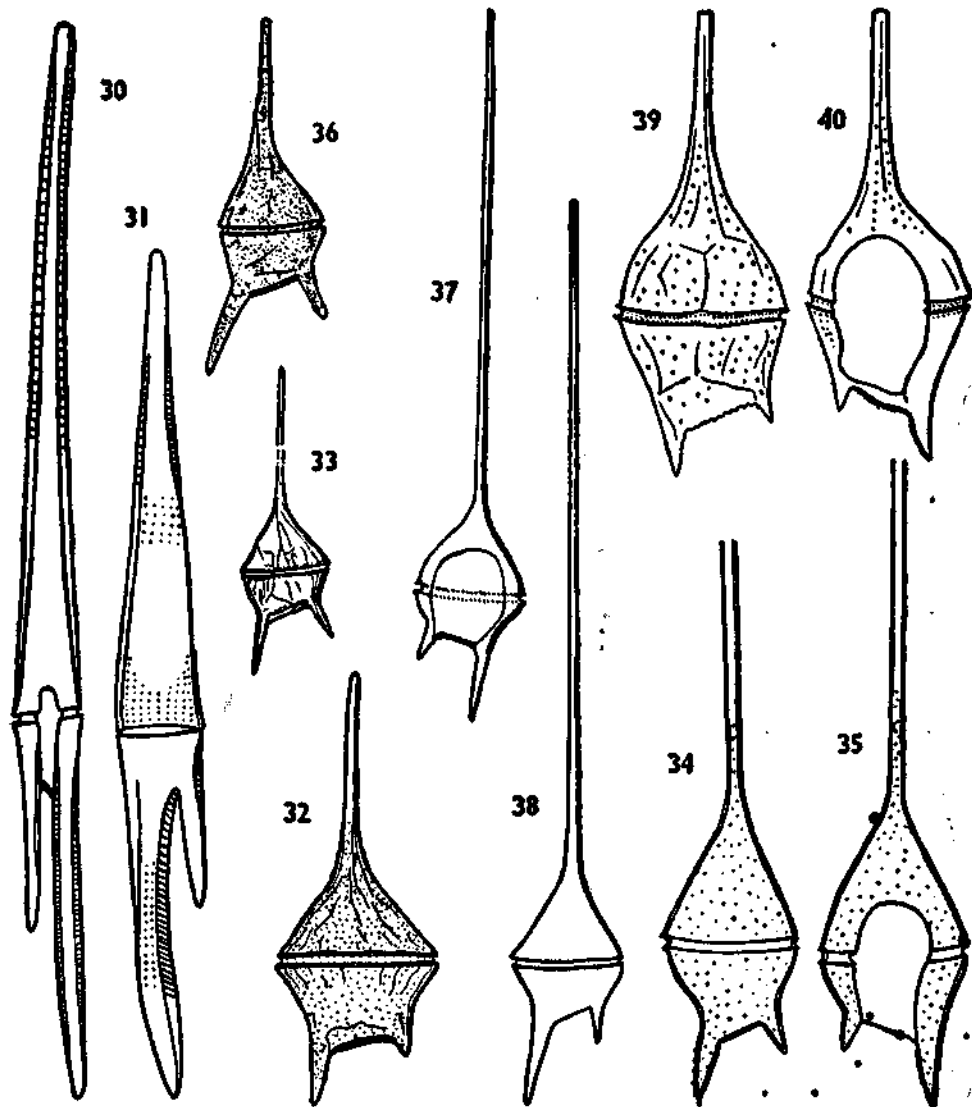
Text-figures 30 - 40. Fig. 30. Ceratium belone Cleve; ventral view; (after Jörgensen) Fig. 31. C. incisum (Karsten) Jörg.; dorsal view; (after Jörgensen, 1920). Figs. 32, 33. C. pentagonum Gourret; dorsal view; (after Böhm, 1931 b). Figs. 34, 35. C. teres Kofoid; dorsal and ventral views; (after Schiller, 1937). Fig. 36. C. lineatum (Ehrenb.) Cleve; dorsal view; (from Schiller, 1937). Fig. 37, 38. C. setaceum Jörgensen; ventral and dorsal views; (36, after Jörgensen; 37, from Schiller 1937). Figs. 39, 40. C. minutum Jörgensen; dorsal and ventral views; (after Lebour, 1925). (30, x250; 31, 36, 37, 38, x340; 32, 33, not known; 34, 35, x 250; 39, 40, circa x 390).
