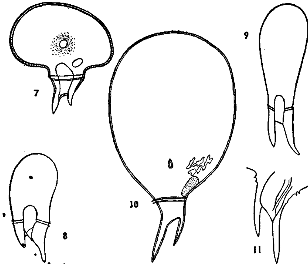
Text Figures 7-11. Fig. 7. Ceratium cephalotum (Lemm.) Jörg; ventral view From Schiller, 1937. Figs. 8 and 9. C. praelongum (Lemm.) Kofoid; ventral views. After Wood, 1963 b. Figs. 10 and 11. C. gravidum Gourret; dorsal and ventral views of posterior end with posterior horn; from Schütt, 1895. (Figs. 7, x 280; 8 and 9, not known, 10, x 230 and 11, x 300).
