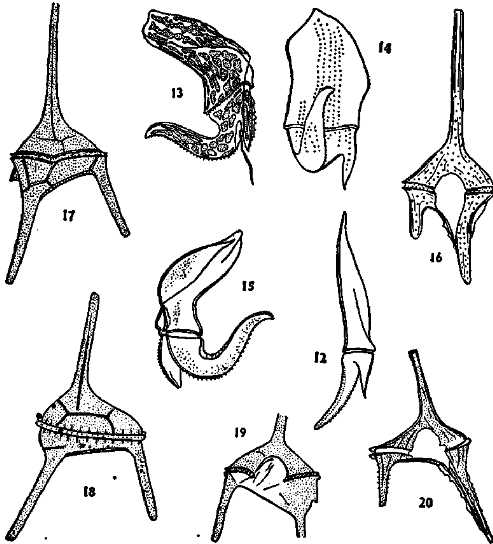
Text-figures 12-20. Fig. 12. Ceratium schroeteri B. Schroeder; dorsal view. From Schiller 1937. Figs. 13, 14, 15. C. digitatum Schütt. 13 and 15, lateral view; 14, dorsal view. 13 and 14, after Schütt, 1895; 15, after Jörgensen.
