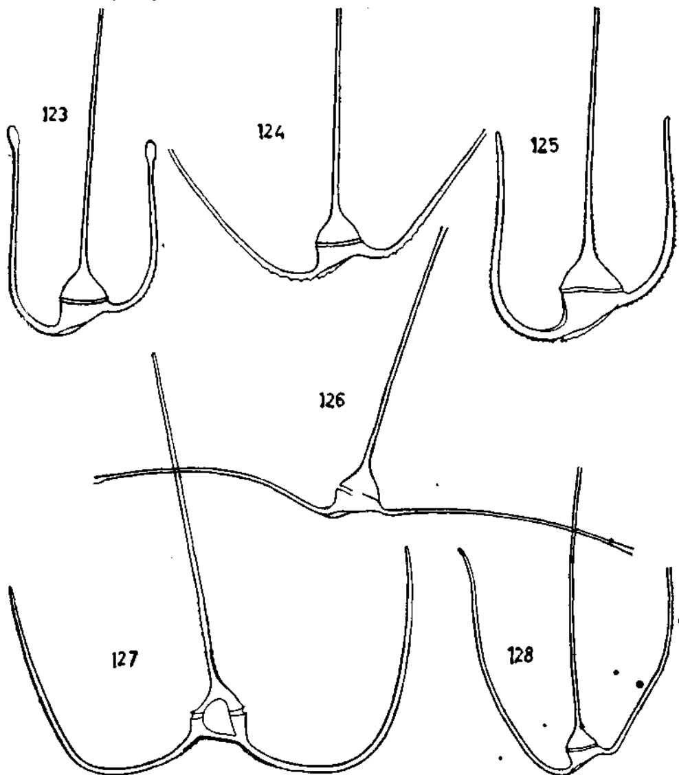
Text-figures 123 - 128. Ceratium horridum Gran. Different specimens of the species. 127, ventral view; (original). Rest dorsal views, (from Schiller 1937). (123, 125, 126, x 210; 128, x 125, 127, x 150. 124 - not given).
