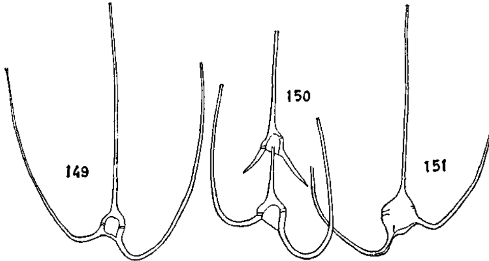
Text-figures 149 - 151. Figs. 149, 150 - Ceratium macroceros (Ehrenb.) Cleve; ventral views; (from Schiller, 1937). Fig. 151 - C. macroceros var. gallicum (Kofoid) Jörgensen; dorsal view; (from Schiller, 1937). (149, 150-x 100; 151-x 200).
