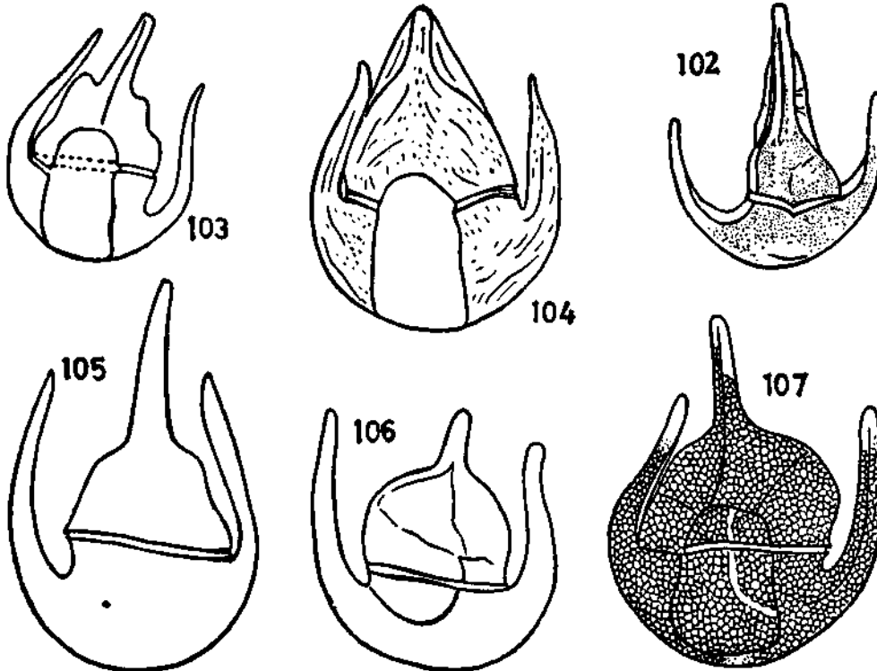
Text-figures. 102 - 107. Fig. 102- Ceratium azoricum Cleve; dorsal view; (from Schiller, 1937). Figs. 103, 104, 105 - C. limulus Gourret. 103 and 104, ventral views, 105, dorsal view; (103, after Jörgensen; 104 and 105, from Schiller, 1937). Figs. 106 and 107 - C. paradoxides Cleve; dorsal and ventral views; (106, after Wood, 1963 a, outline only; 107, after Jörgensen, 1920). (102, 103, 105, x 350; 107, x 310; 104, 106, not known).
