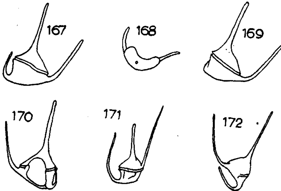
Text-figures 167 - 172. Ceratium egyptiacum Halim. Fig. 168 - apical view; 170 & 172 - ventral views; rest dorsal views. (167 - 170, after Halim, 1963; 171 & 172, after Halim, 1965; magnification not given).
