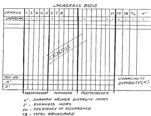
Fig.1 Data matrix for community organisation studies on sub-habitats.
