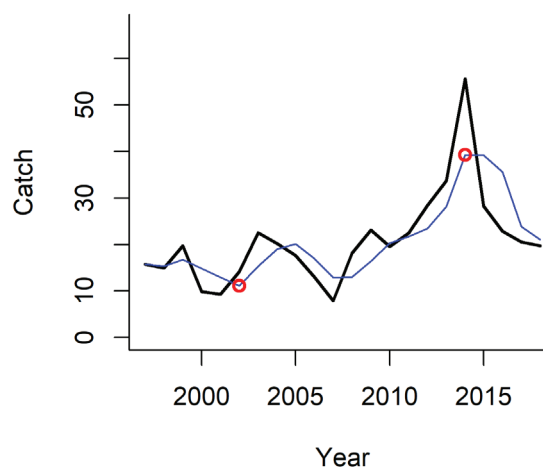
Fig. 1a. Time series of Indian mackerel landings during 1997-2018 (Blue line is the three year moving average, maximum and minimum landings are denoted with red dots)
