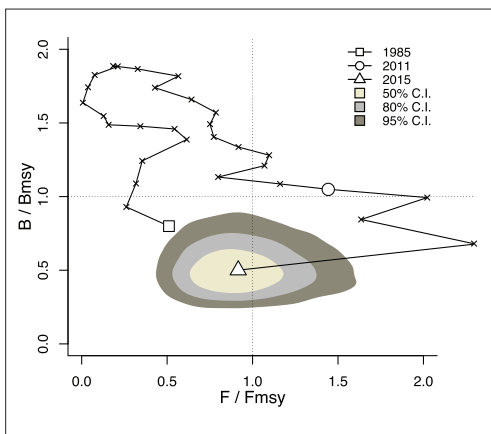
Fig.52. Reference points for biomass ( B/B_{MSY} ) and fishing levels ( F/F_{MSY} ) of Indian oil sardine on the southwest coast during 1985 - 2015
