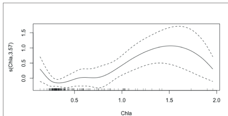
Fig.62. Relationship between Chl a and the recruitment success for Indian oil sardine using GAM model.
