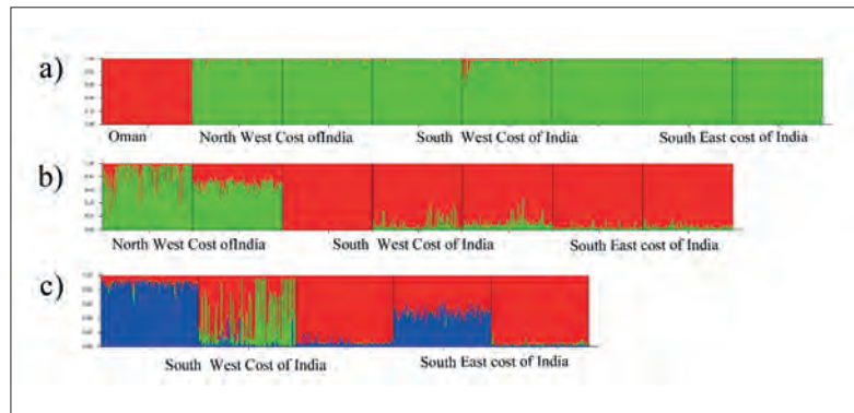
Fig.60. Graphical results of STRUCTURE analysis of six microsatellite loci in Indian oil sardine populations. Vertical lines represent probability of individual membership in simulated clusters. a) Plot for K = 2 (including all the samples), b) Plot for K = 2 (excluding Oman samples), and c) K = 3 (Excluding Oman and Northwest coast of India samples).
