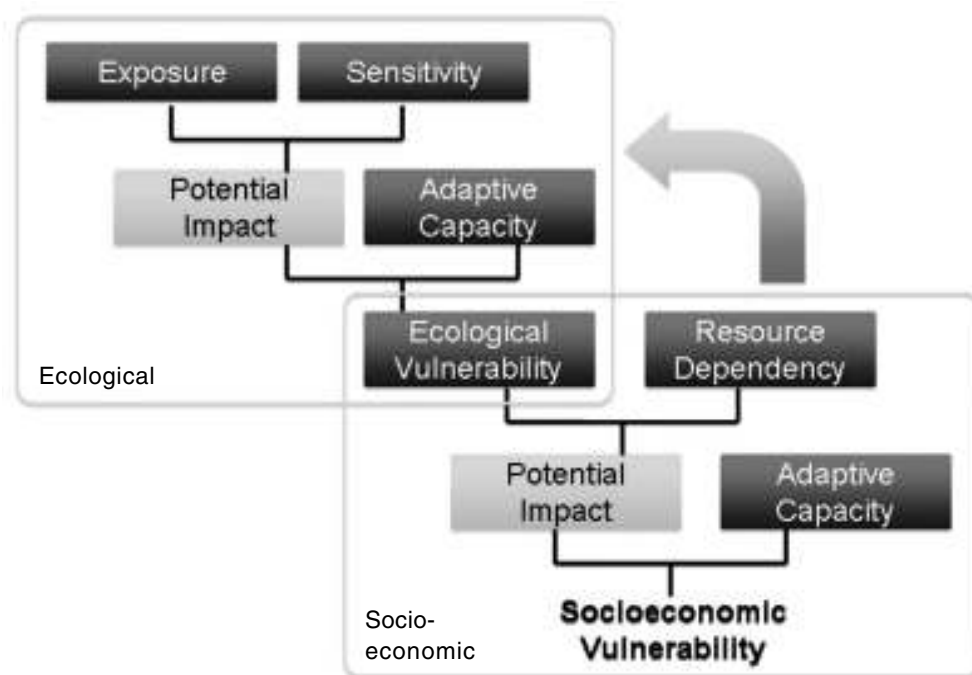
Fig. 6. Vulnerability model
