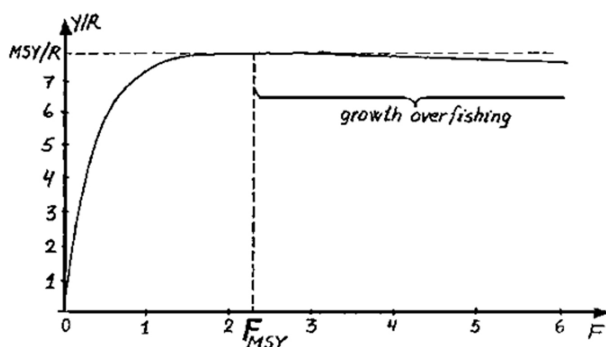
Fig. 3. A typical Y/R curve as a function of Fishing mortality
