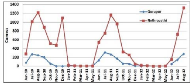
Fig. 2 Discharge rates of Gurupur and Nethravathi rivers
